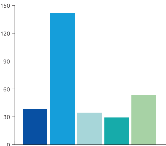
Per capita anthropogenic emissions of methane and black carbon in different source regions in 2010
