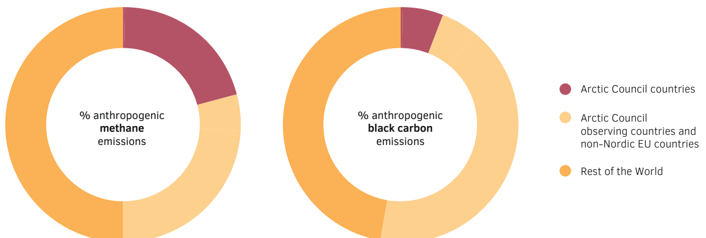
Origin of global (2010) emissions of methane and black carbon from anthropogenic sources
