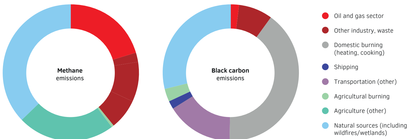
Sources of global (2010) emissions of methane and black carbon
