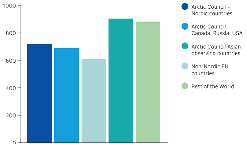
Per capita anthropogenic emissions of methane and black carbon in different source regions in 2010
